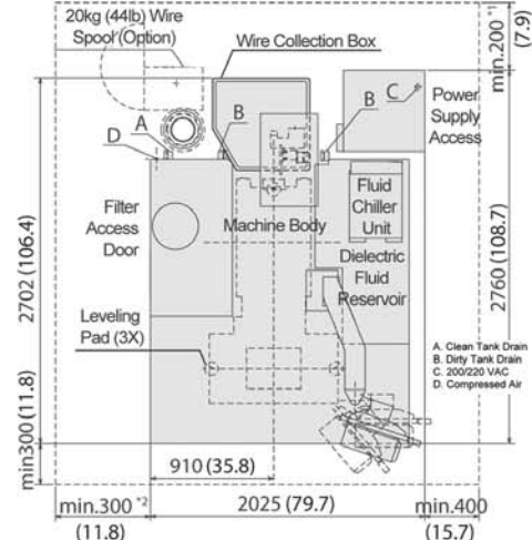
MV1200-R Layout Drawing
