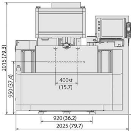
MV1200-R Layout Drawing
