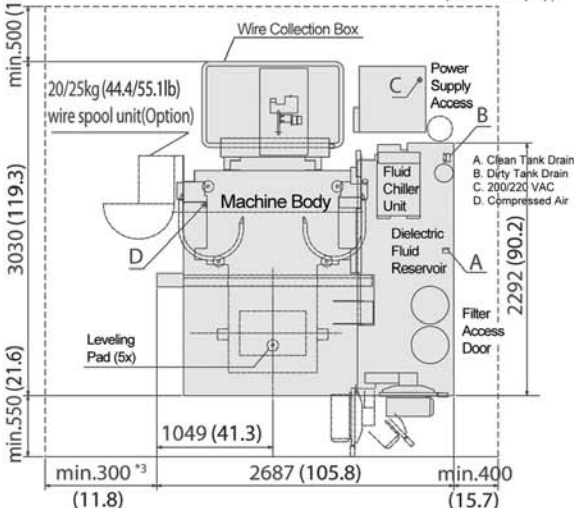
MV2400-S Layout Drawing
