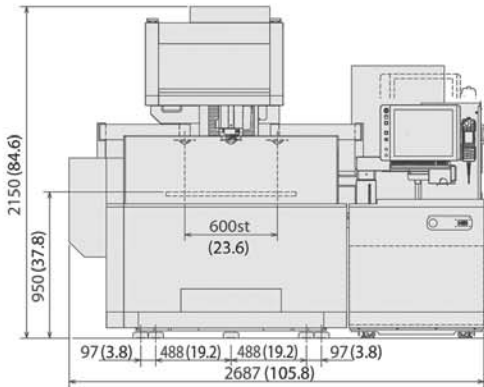
MV2400-S Layout Drawing
